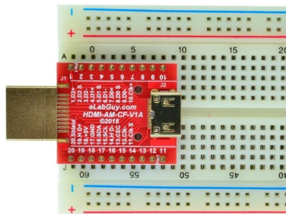
Figure 2: Example of connecting the HDMI-AM-CF-V1A on a proto PCB (Note: This picture only shows the pins spacing, actual use may not be used on a breadboard)
